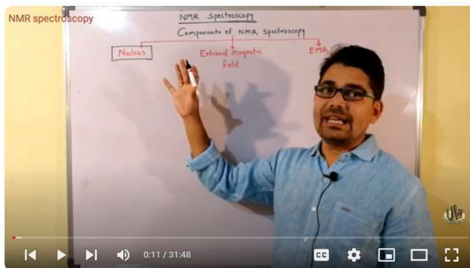
Lecture 2 Principle of NMR Spectroscopy/Why we use Radio Frequency as a source of EMR
